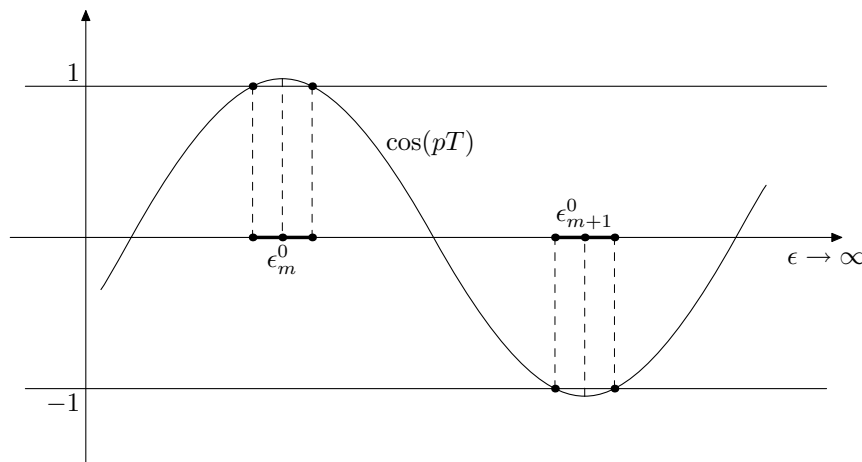
Figure 3: For the generic T -periodic potentials the gaps are located near the points \epsilon_m = 4\pi^2 m^2 T^{-2} for \epsilon \rightarrow \infty . Here m are the integer numbers.
