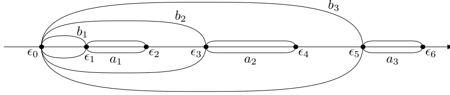
Figure 5: The canonical basis of cycles (a_i, b_j) on the Riemann surface \Gamma with branching points \epsilon_0, \dots, \epsilon_{2n} . (Here n = 3 )
