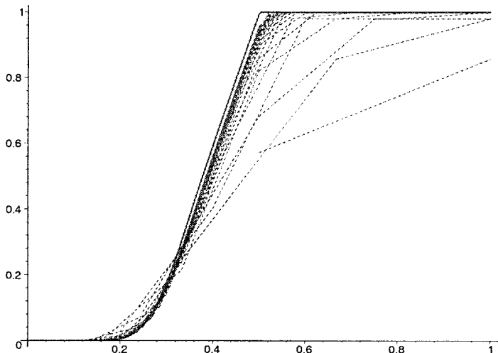
FIG. 6. A plot of the “density” of the largest irreducible factor degree for polynomials of \mathbb{F}_7[x] . The representation of (xn)\Pr(D_1 = xn) , for degrees n = 1, \dots, 25 and x \in [0, 1] (dashed lines), shows fast convergence against the limit f(x) (continuous curve).
