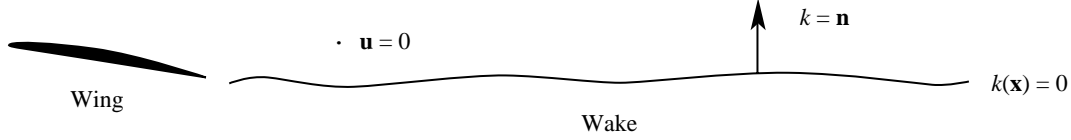
Figure 7. Thin wing in incompressible, irrotational flow with wake.
